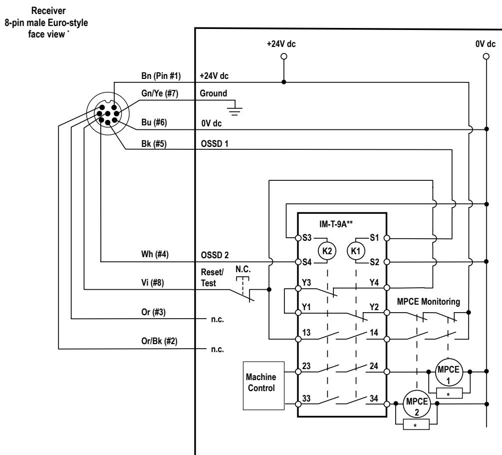
Figure 22. Generic Wiring — Interface Module (2-Channel EDM, Manual Reset)
