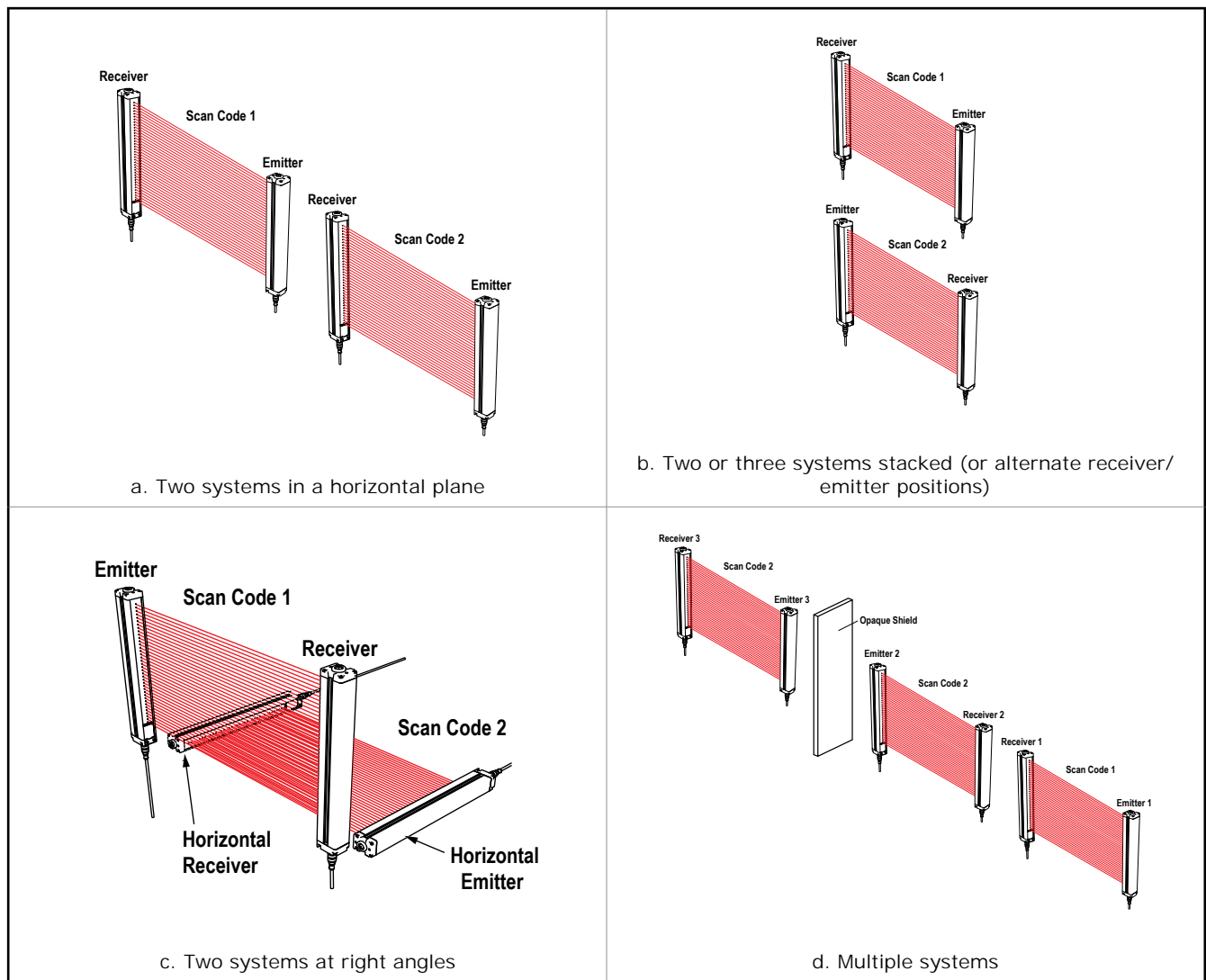
Figure 9. Installation of Multiple Systems
