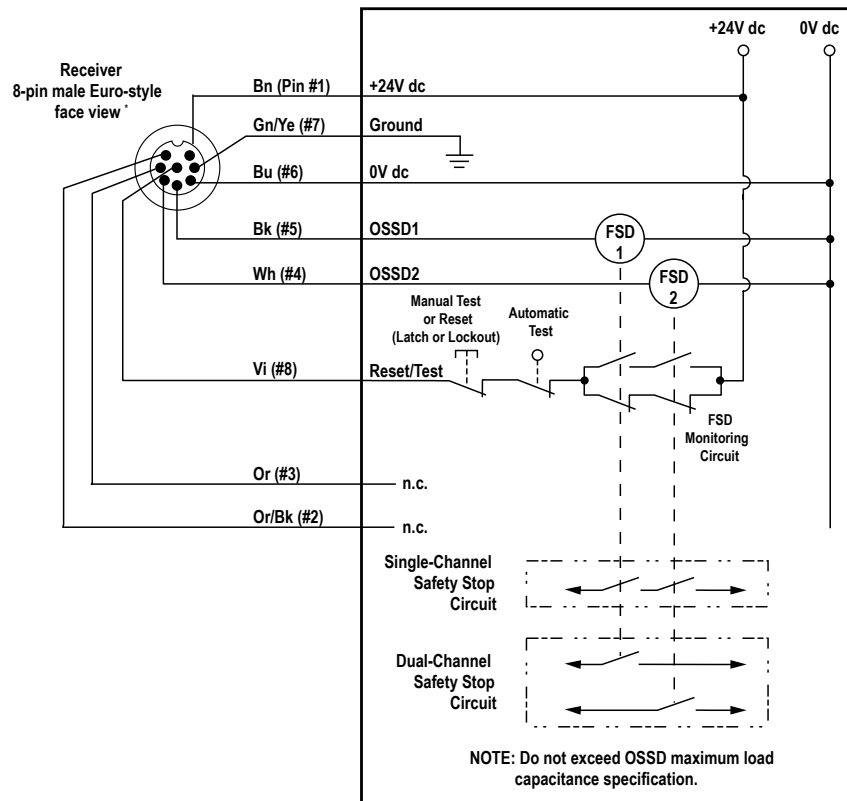
Figure 21. Generic Wiring to FSDs (manual reset)
