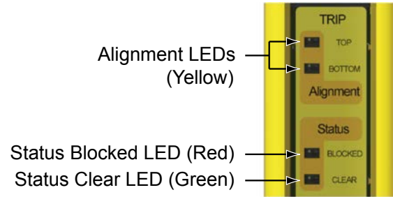
Figure 15. Receiver Status Indicators
