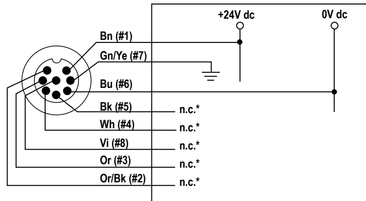
Figure 20. Emitter—Generic Wiring Diagram
