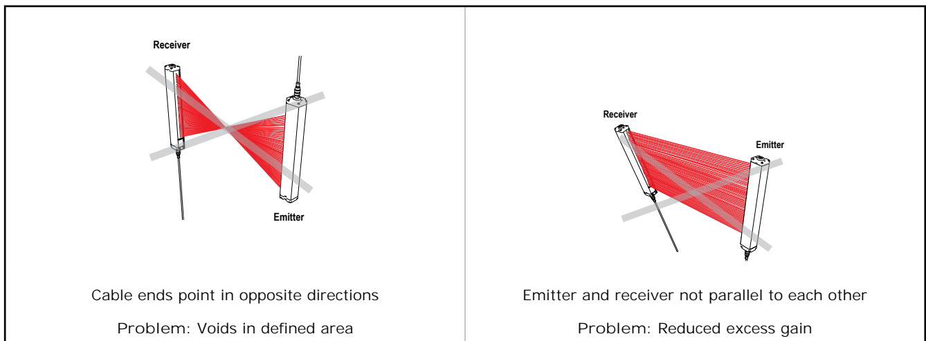
Figure 8. Examples of Incorrect Emitter/Receiver Orientation
