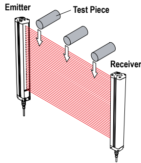
Figure 18. Trip Test
