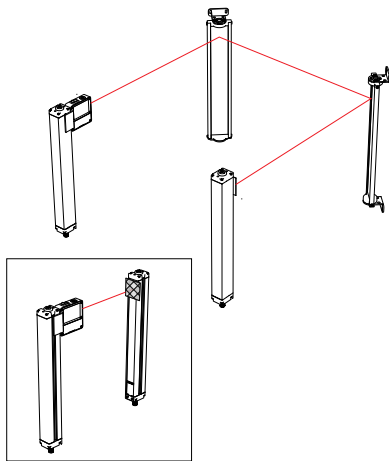
Figure 16. Optical alignment using the LAT-1-LS
