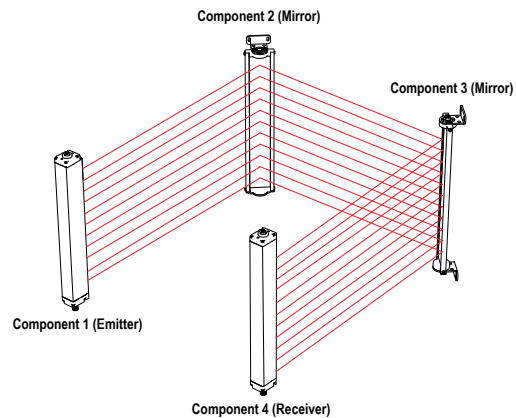
Figure 17. Corner Mirror Alignment
