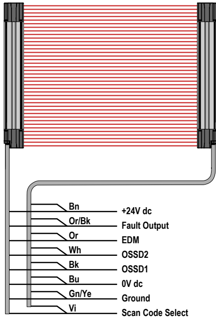
Figure 12. Individual cordsets
