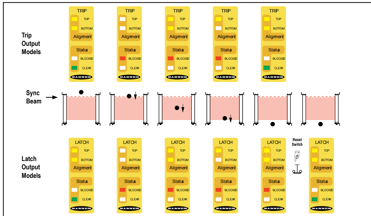
Figure 23. Status Indicator behavior during the trip test
